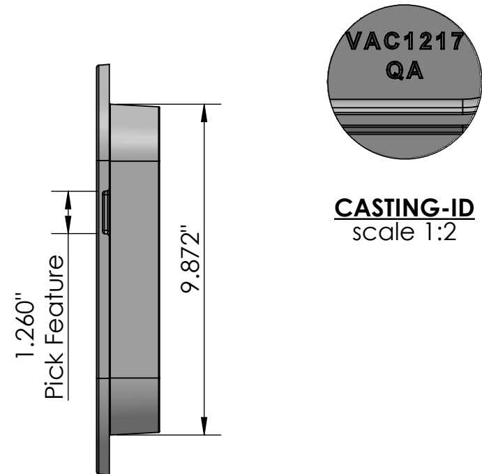
END VIEW scale 1:4
