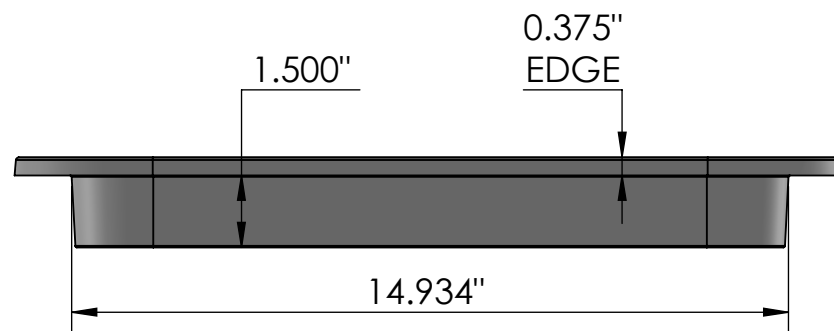
SIDE VIEW scale 1:4
