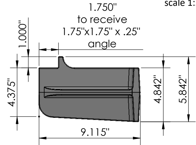
END-VIEW scale 1:5
