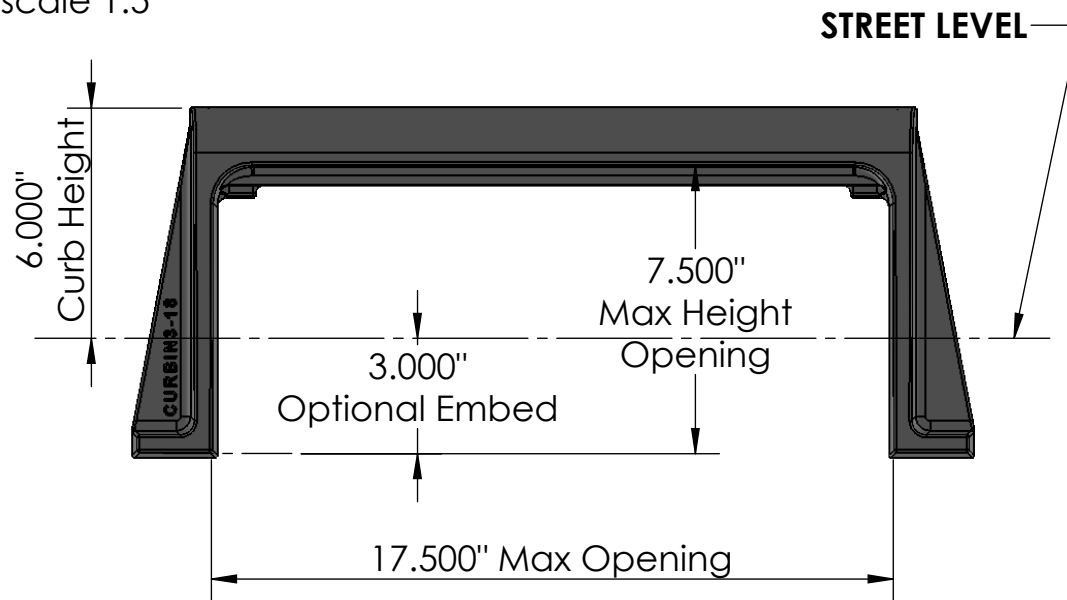
SIDE VIEW scale 1:5
