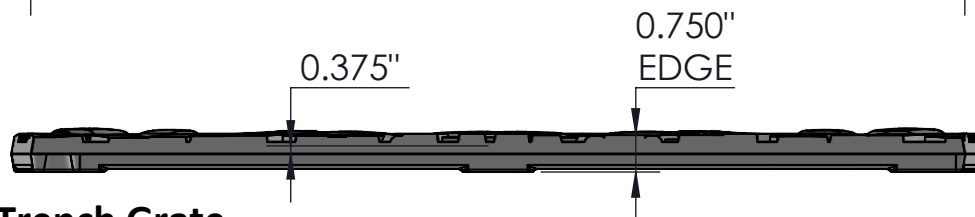
SIDE VIEW scale 1:4
