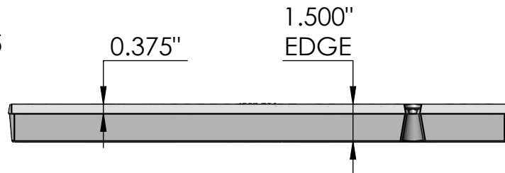
SIDE VIEW scale 1:5.5
