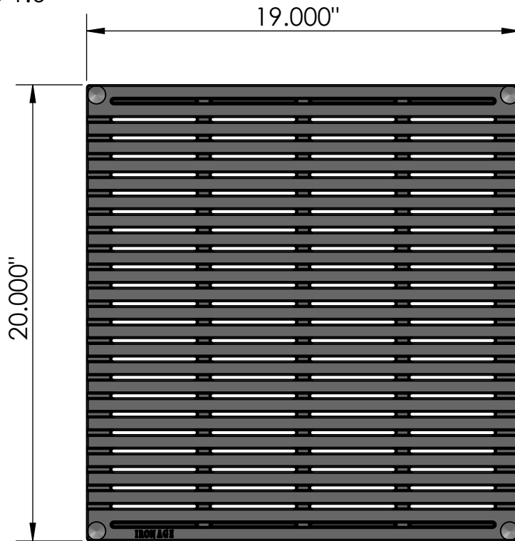
TOP VIEW scale 1:6
