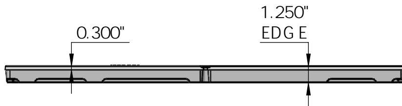
SIDE VIEW scale 1:7
