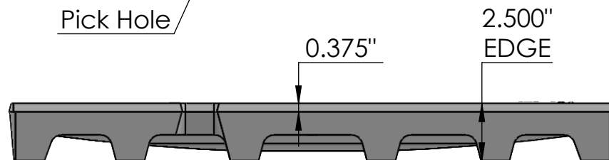
SIDE VIEW scale 1:6
