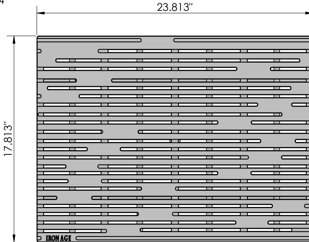
Bottom VIEW scale 1:10
