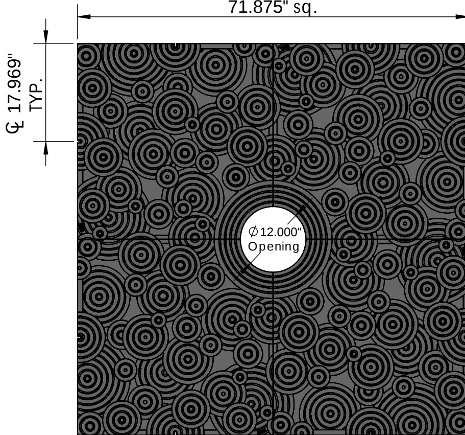
TOP VIEW scale 1:18
