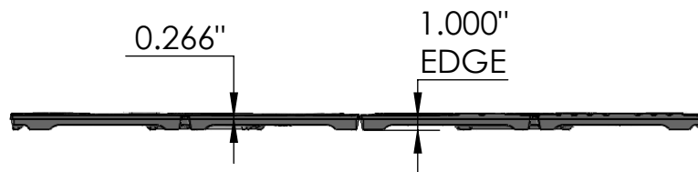
SIDE VIEW scale 1:12
