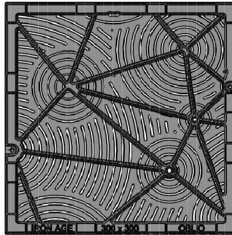
BACK scale 1:5
