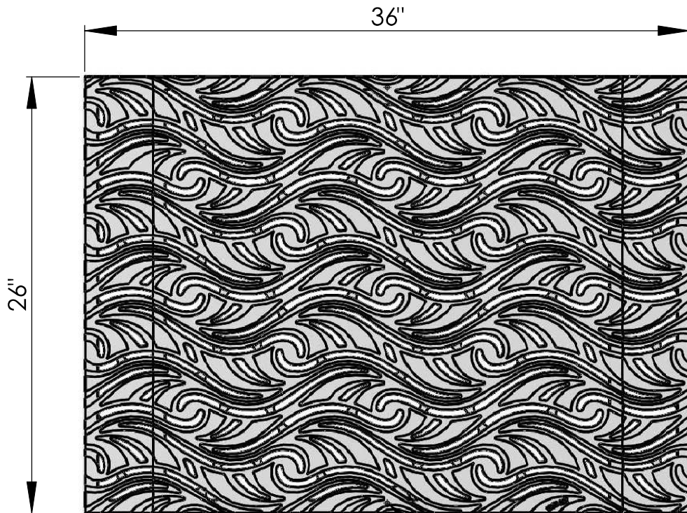
TOP scale 1:8
