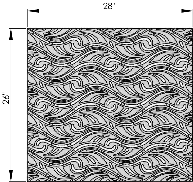
TOP scale 1:8
