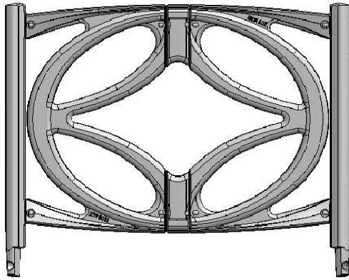
INTERLAKEN 2'x2' PLANTING FENCE scale 1:10
