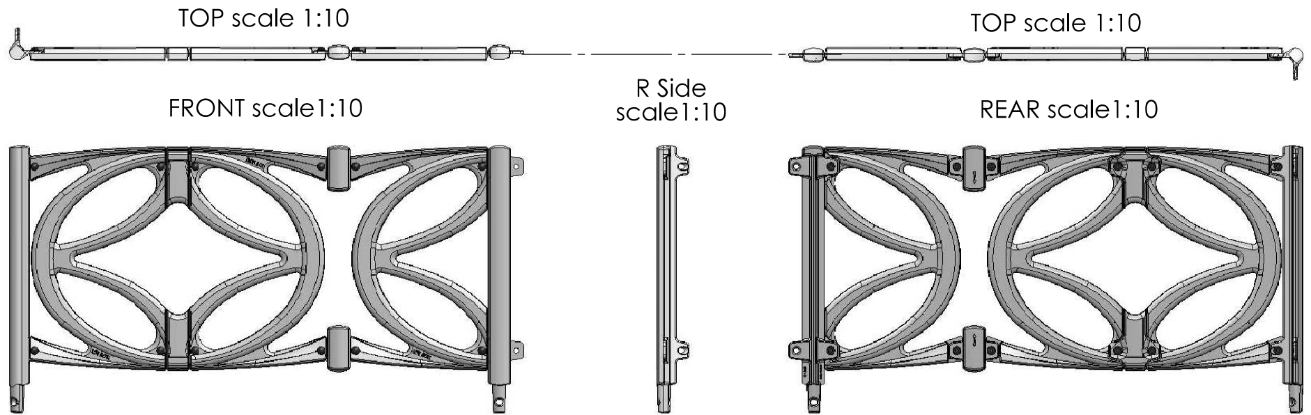
FRONT EXLODED scale 1:10
