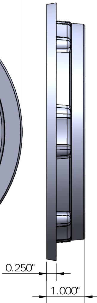
SIDE VIEW scale 1:1.5
