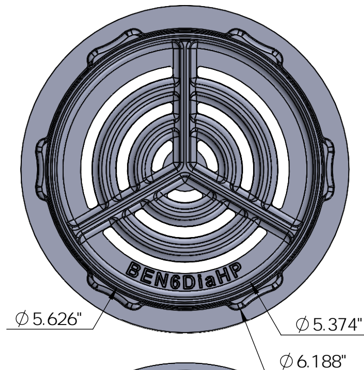
Bottom View scale 1:2
