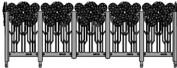
DAISY 3'x5' PLANTING FENCE scale 1:20
